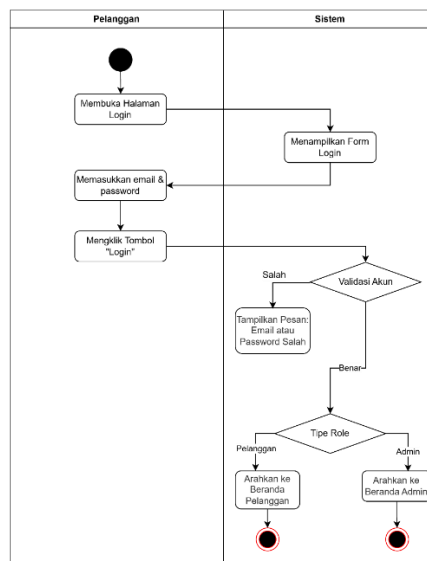
Activity Diagram: Login
