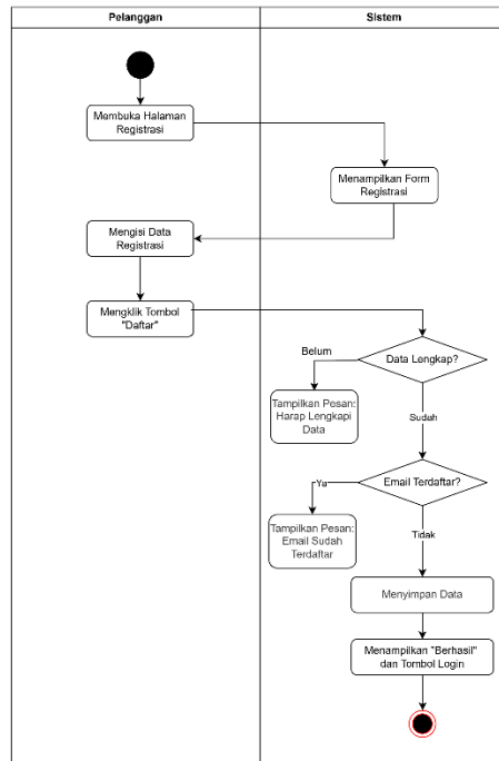
Activity Diagram: Registrasi
